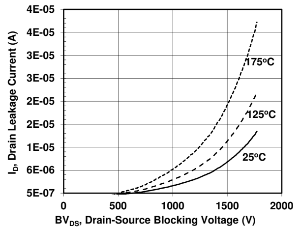
Figure 12. Drain-Source Leakage
